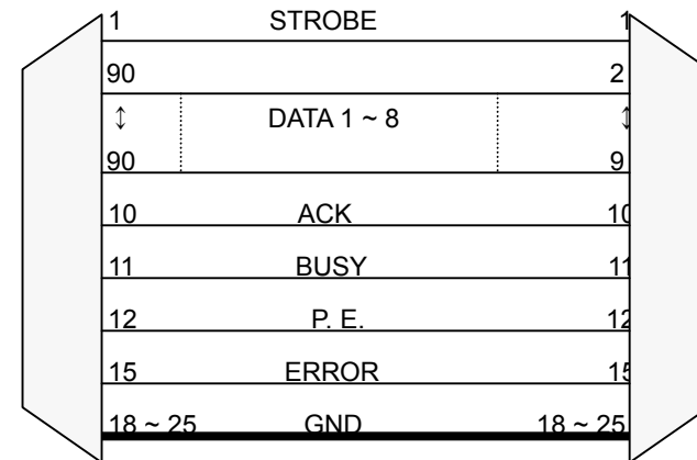
25 Pin D-SUB Connector (MALE) HOST
